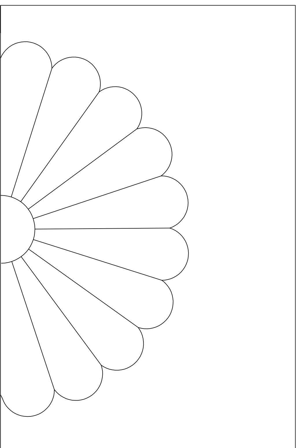
View: Full Size Template of Center Drawer Front with Carved Shell
